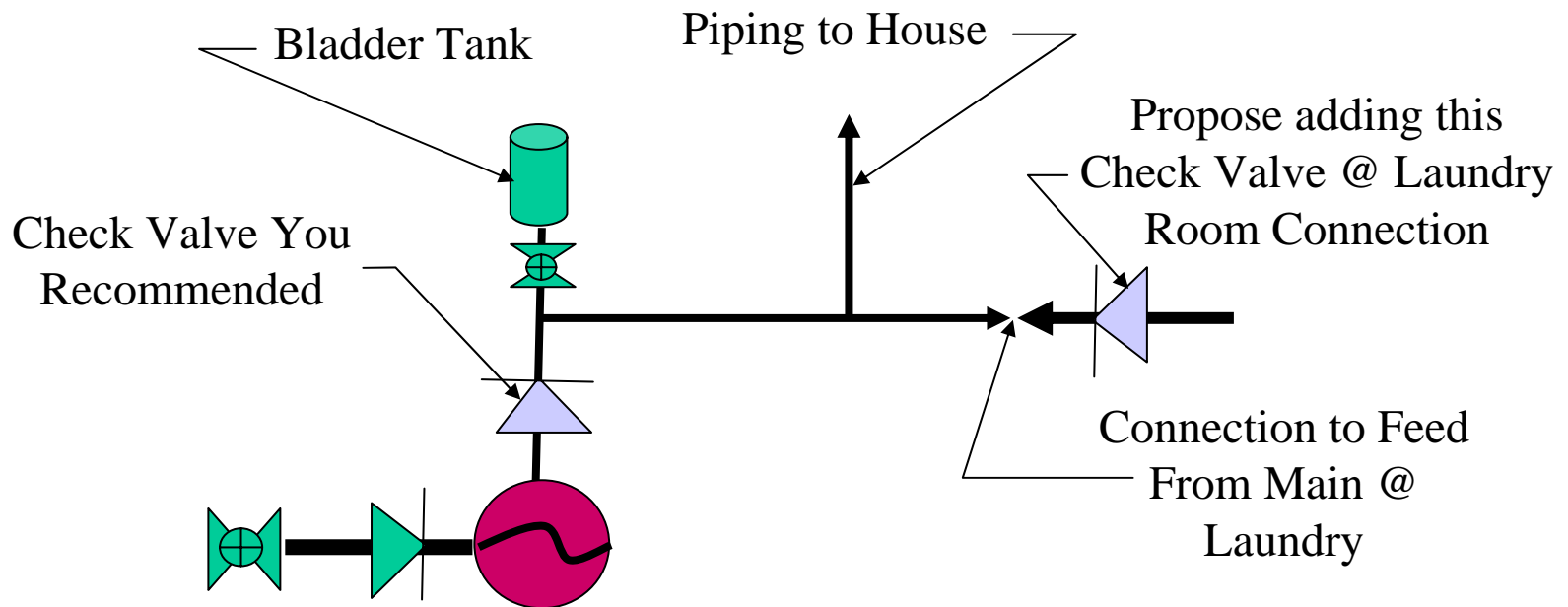
Booster Pump Configuration
