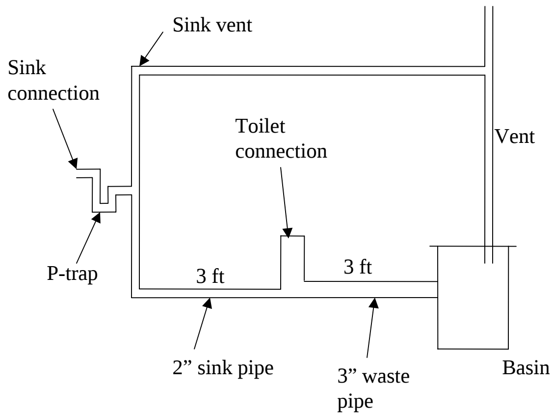
Plumbing diagram
