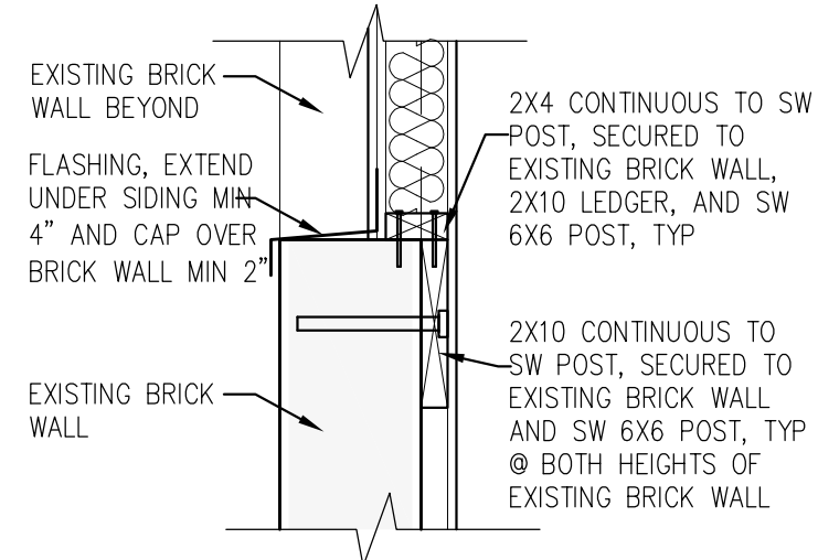
DETAIL: LEDGER BOARD
