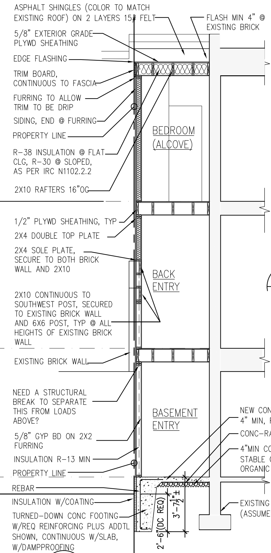
SECTION (EAST/WEST)
