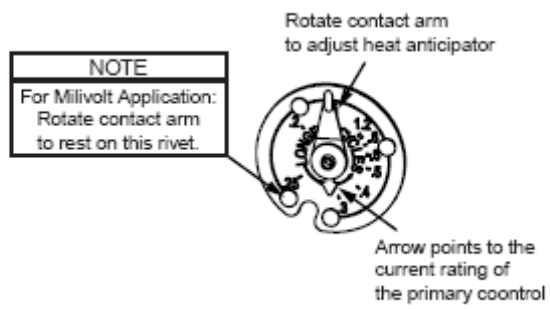
Figure 5. Anticipator adjustment
