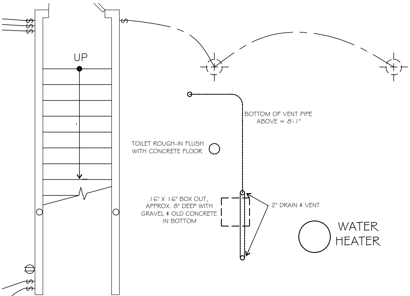
PARTIAL BASEMENT PLAN
