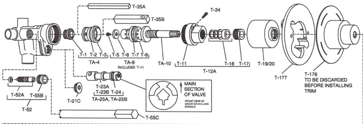
FIGURE 9 Parts Breakdown
